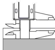
Offset Measurement
