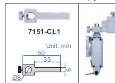
dial test indicator holder (optional)
